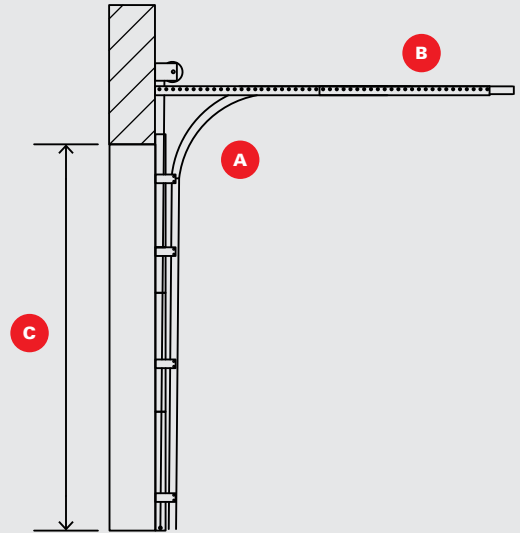
DOOR SIDE VIEW
